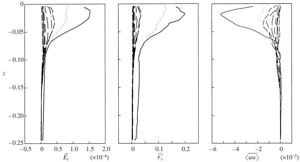
FIGURE 13. Averaged horizontal profiles of the mean turbulent kinetic energy, \bar{E}_t , the mean square turbulent vorticity, \bar{V}_t^2 , and the Reynolds stress, \langle uw \rangle . Note that the horizontal average is over a length of 0.7 defined by the vertical lines in figure 9 which move at the speed of the turbulent cloud.
