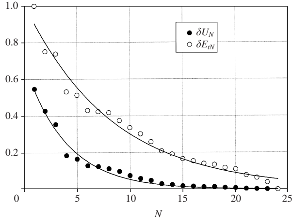
FIGURE 4. Examples of convergence of the normalized ensemble-averaged velocity magnitude, ●, and the corresponding normalized turbulent kinetic energy, ○, based on a total sample size of 24 repeats. The data shown in this paper were computed for production runs of 15 repeats, giving relative errors of approximately 2% and 16%, respectively.
